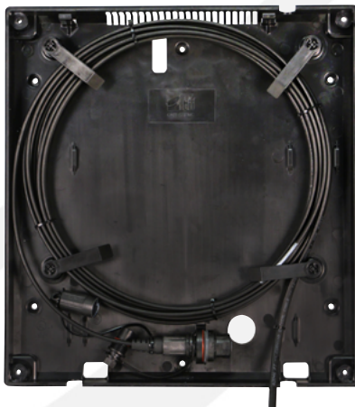
ONT-SSENC1 shown with OSP drop cable and OptiTap™ to SC Adapter (not included)
